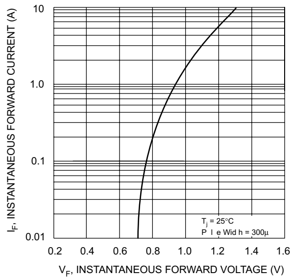
Fig. 2 Typical Forward Characteristic (Element)
