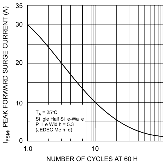
Fig. 3 Maximum Peak Forward Surge Current (Element)
