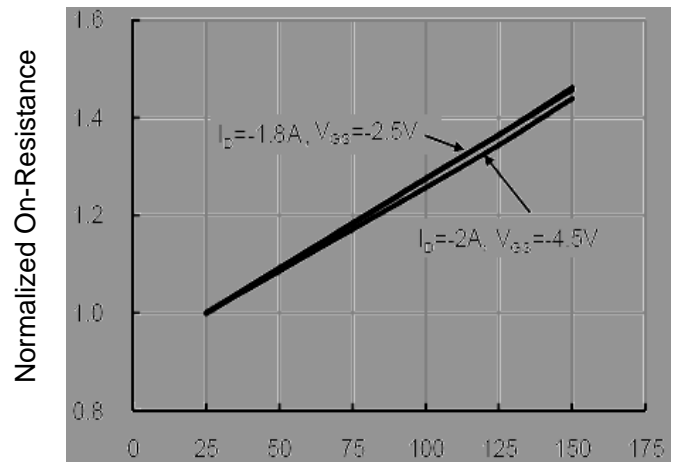
Figure 4 Drain-Source On-Resistance
